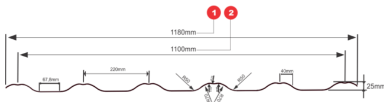
1 - Total width 2 - Effective width
